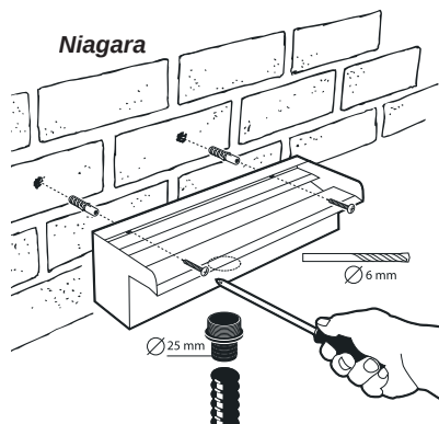
Niagara LED 30
